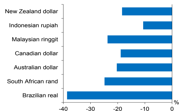
Figure 3.9 Commodity currencies against the USD (% change since January 2014)
