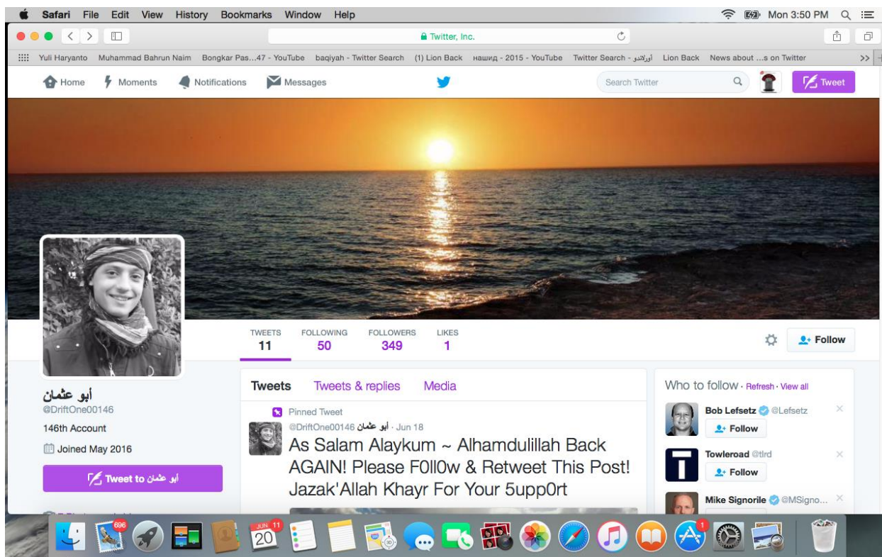
Figure 6: DriftOne00146 posting 06/20/2016
