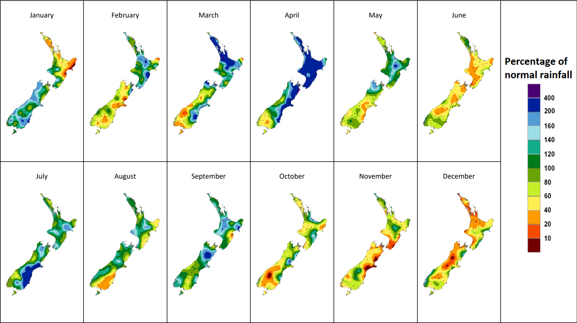
Figure 2: Monthly rainfall as a percentage of the 1981-2010 monthly normals for each month of 2017.
