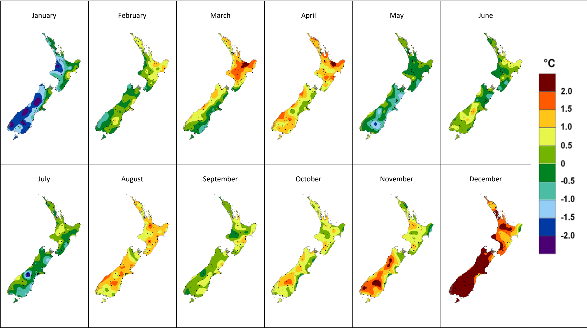
Figure 1: Monthly temperature anomalies (compared to the 1981-2010 monthly averages) for each month of 2017.
