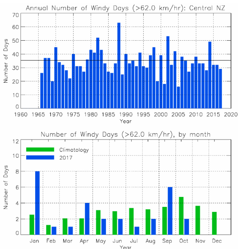
Figure 3: (above) Annual number of ‘windy days’ for central New Zealand, 1966 to 2017, with horizontal line indicating the 1981-2010 average (35.3 days); (Bottom) Number of ‘windy days’ by month, comparing the months of 2017 (blue histogram) with the 1981-2010 average (green).
