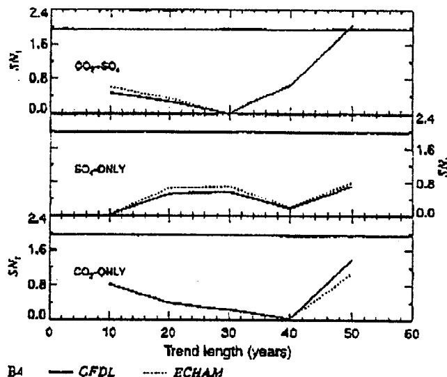
of the coupled-model differences in the spectral density of global-mean, annually averaged temperature on time scales of 10- to 50 years (see Fig. B2). The thin solid line gives the 5% significance threshold for an assumed Gaussian distribution of trends
