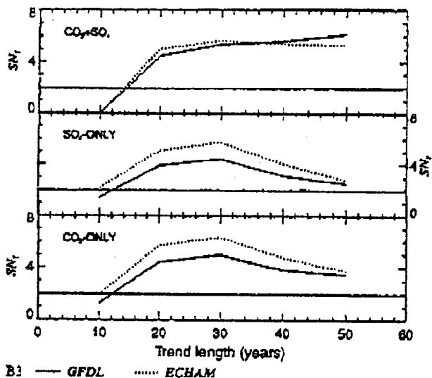
Fig. B3. Signal-to-noise ratios, SN_i , for observed trends in the un-centered pattern correlation statistic C(t) . The signals, \beta_S(t) , are the observed trends in C(t) for the last 10- to 50 year. The noise, \epsilon_N(t) , is the standard error of the sampling distribution of \beta_N(t) (see Sect. 6.1 and Appendix B for further details). Standard errors were computed using data from both GFDLCTL and HAMCTL. Results are for annually averaged near-surface temperature data. For temperature-change signals from the Taylor and Penner sulfate-only and CO_2 -only experiments, SN_i is consistently lower for the GFDLCTL noise estimates. The GFDLCTL versus HAMCTL differences in SN_i can be interpreted in terms
