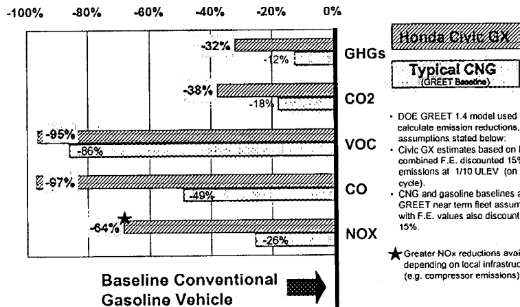
GHG and Emission Benefit Relative to Conventional Gasoline Fleet, %
