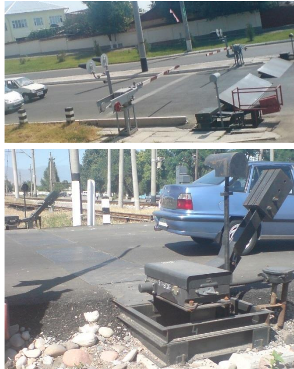
Figure 4-5: Vehicle Barriers at a Railroad Crossing
