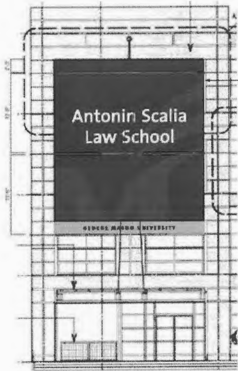
1 HOTEL HILL PARKWAY DRIVE ENTRANCE SIGNING ELEVATION SCALE: 1/8" = 1'-0"
