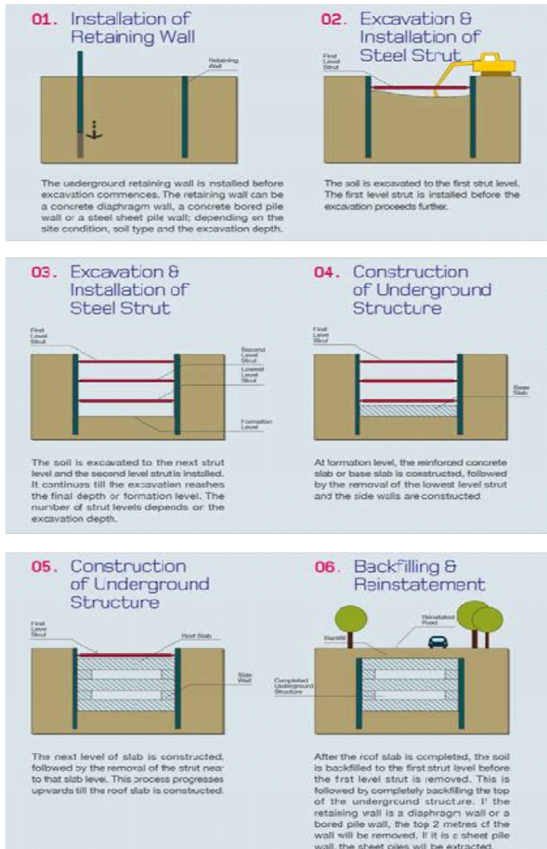
Exhibit 7-5: Cut and Cover Tunnel
