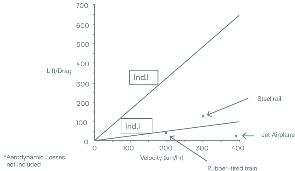
Exhibit 2-6: Inductrack's Lift to Drag Ratios 1
