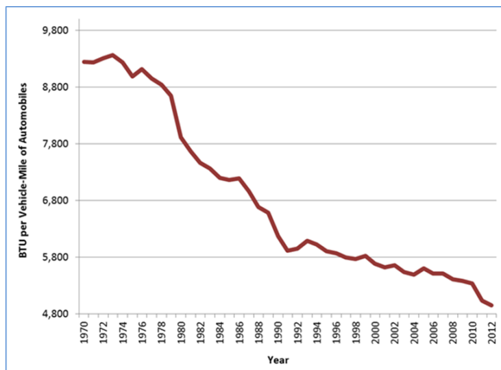
Exhibit 5-3: ORNL Historical Highway Automobile Energy Intensities Data
