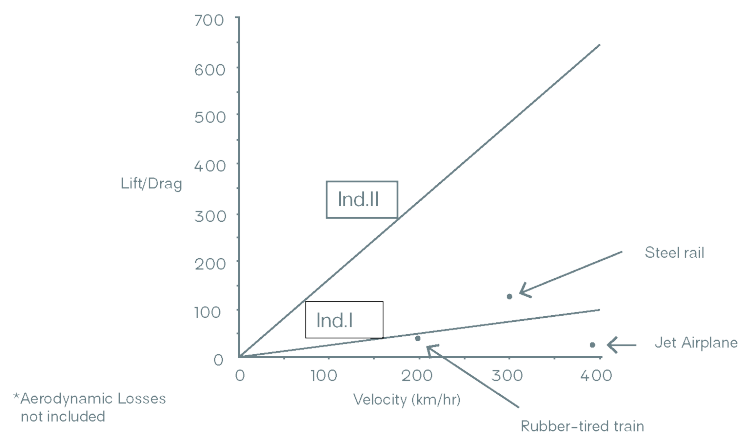
Exhibit 2-6: Inductrack's Lift to Drag Ratios 1
