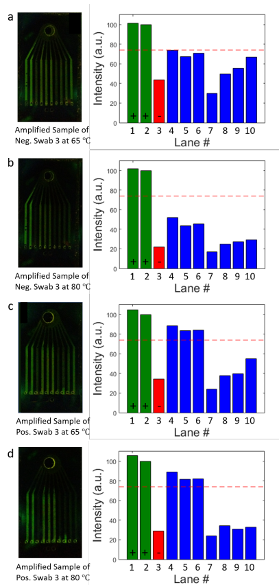
Fig. 4 On-chip tests of horse swab samples. The smartphone pictures of the amplified chip for a negative sample ( \sim 400 EHV1 genome copies/mL) and corresponding average channel intensities were obtained at a) 65 °C and b) 80 °C. The results for a positive sample ( \sim 5.48 \times 10^6 EHV1 genome copies/mL) were also obtained at c) 65 °C and d) 80 °C. Increasing chip temperature at the imaging time decreased background fluorescence from unamplified primers and improved positive/negative contrast. (Reagents dried on the chip for Channel 1: the E. coli positive control primers, Channel 2: the EHV3 positive control primers and DNA, Channel 3: the negative control primers, Channel 4–6: EHV1 primers, Channel 7–10: S. equi , S. zoo , EHV4 and EIV primers, respectively.)
