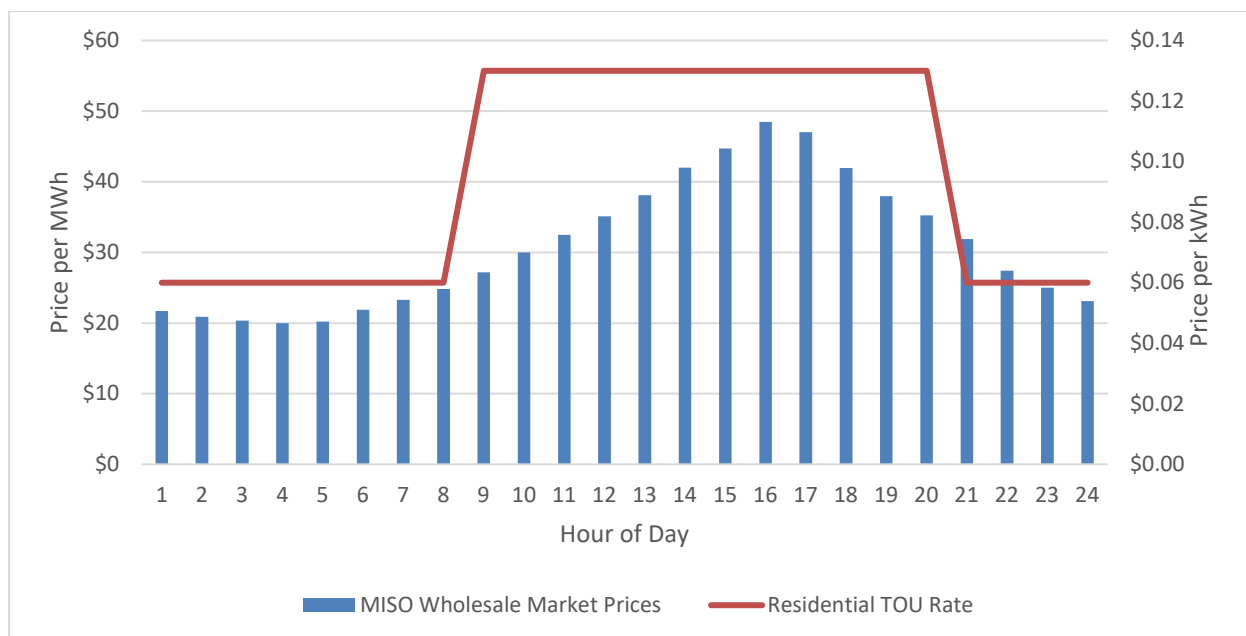
Figure 4-9 Time Varying Price of Electricity on an Average Summer Day in Wisconsin
